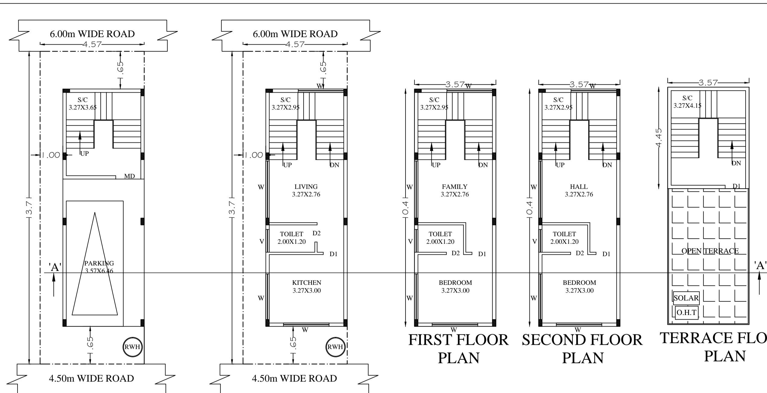
STILT FLOOR PLAN, GROUND FLOOR PLAN, FIRST FLOOR PLAN, SECOND FLOOR PLAN, TERRACE FLOOR PLAN
